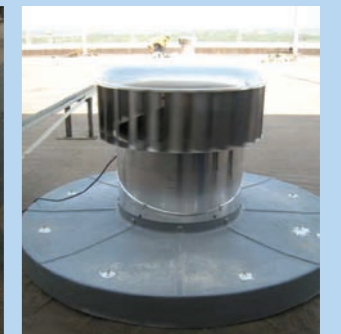
NEW HYBRID VENTILATOR (ECOPOWER EP600)
